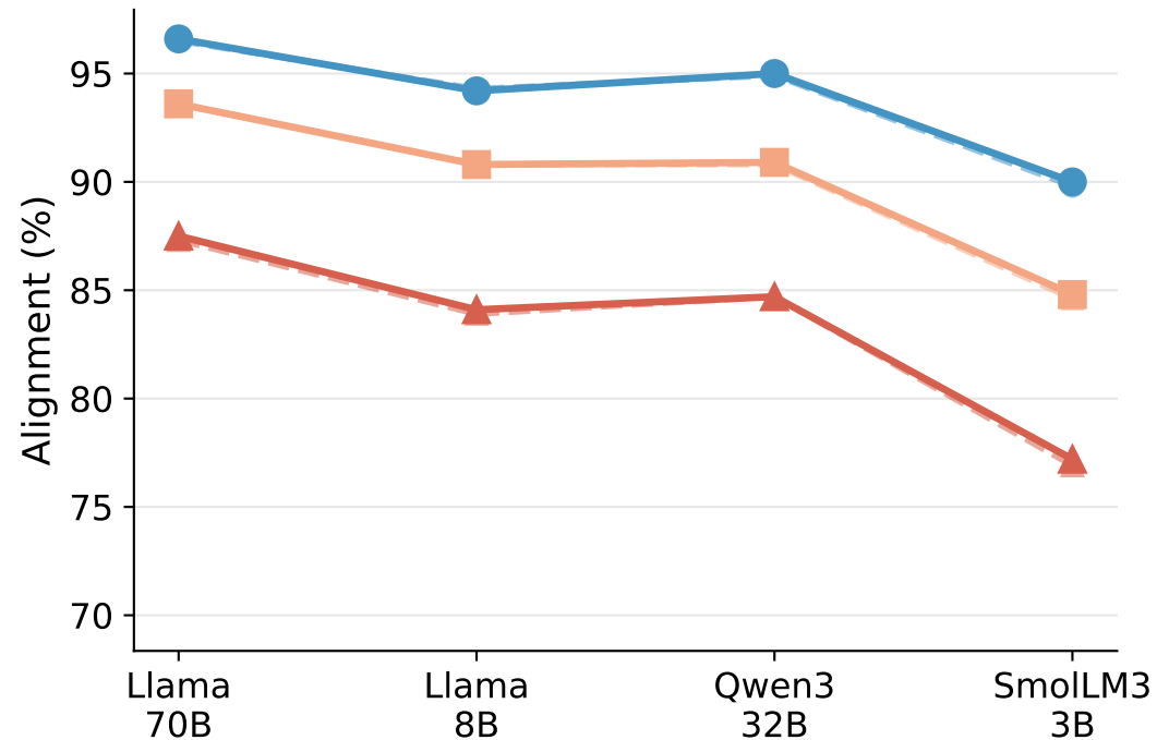
With GT
