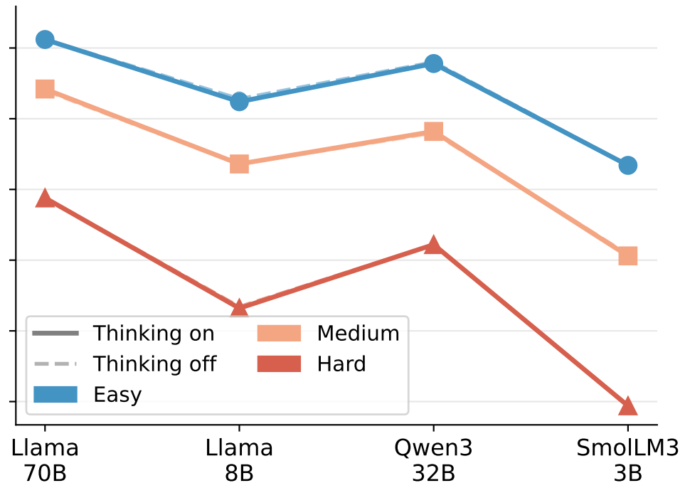
Without GT
